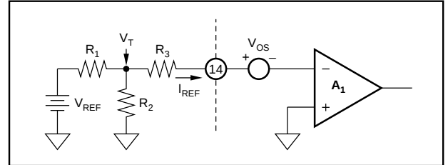
FIGURE 5. "T" Network for Reference Current.
